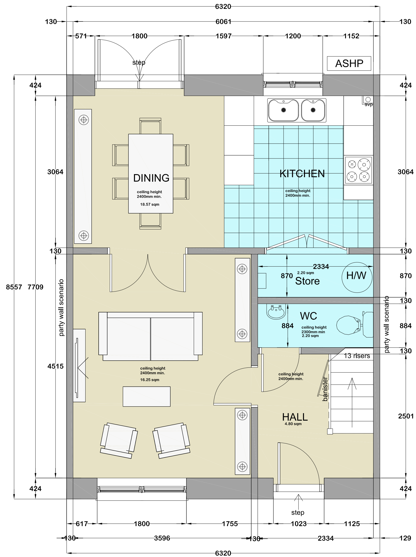
GROUND FLOOR PLAN 3B/5P TH 46.717sqm (500sqft)
