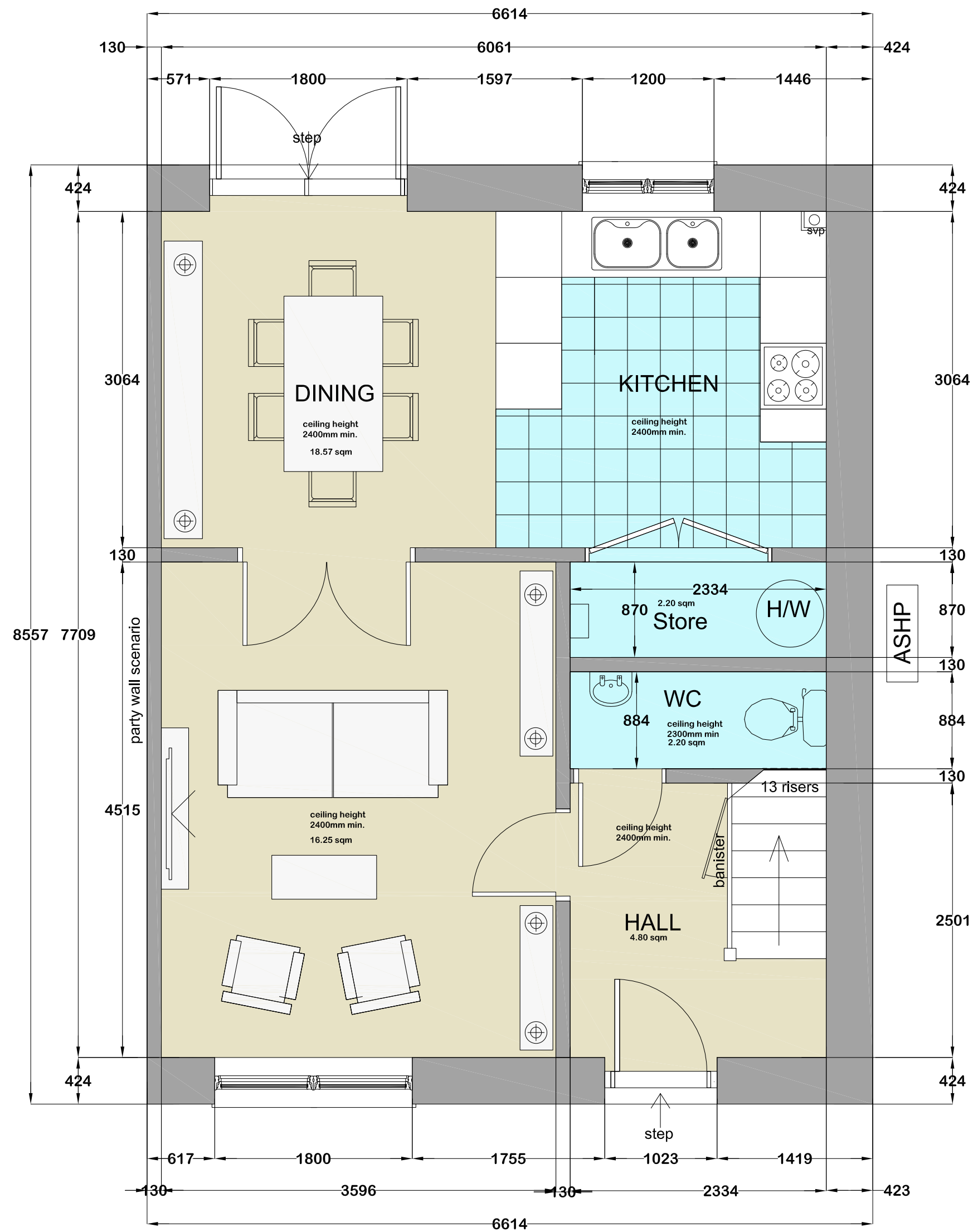
GROUND FLOOR PLAN 3B/5P TH 46.717sqm (500sqft)
