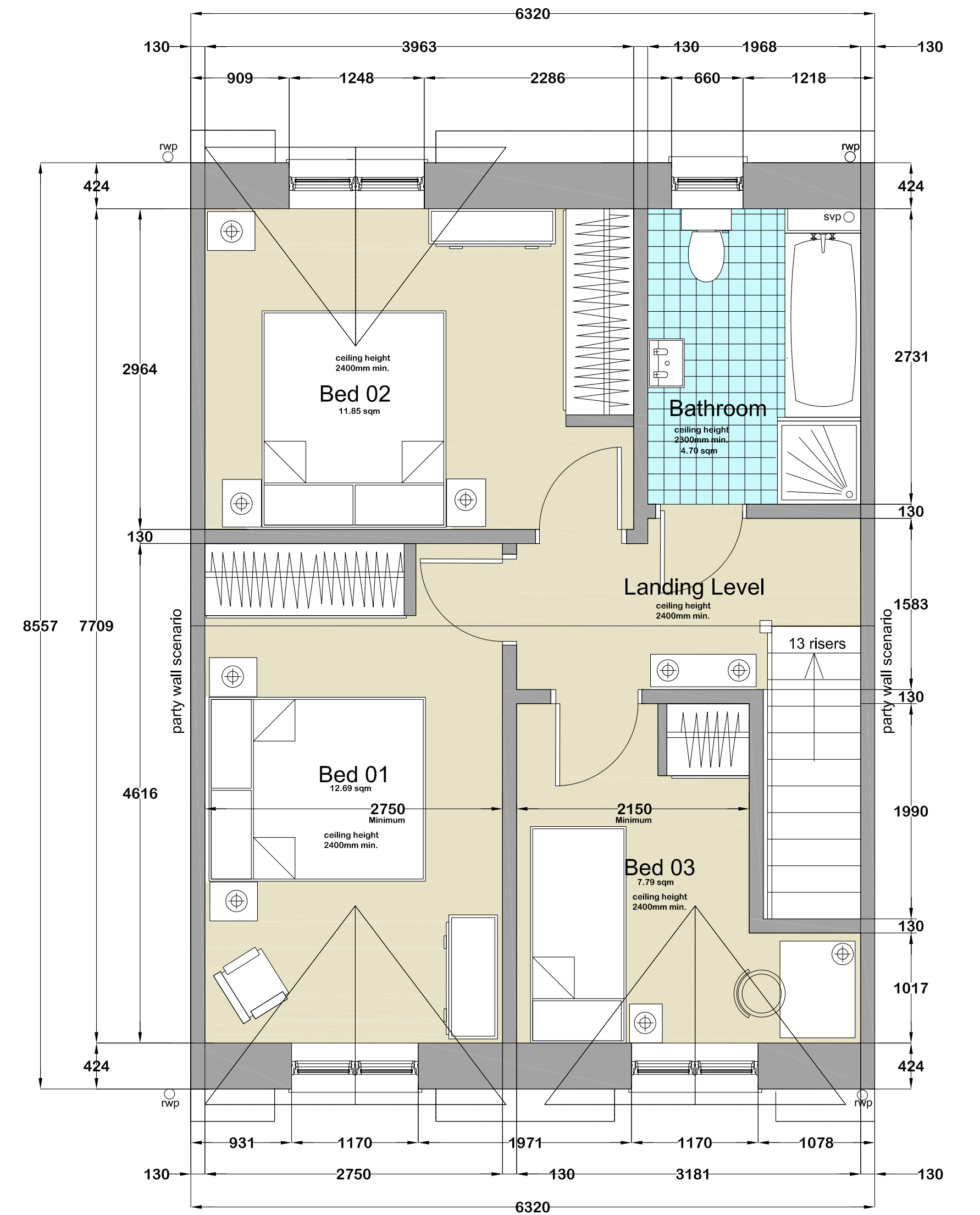
FIRST FLOOR PLAN 3B/5P TH 46.717sqm (500sqft)
